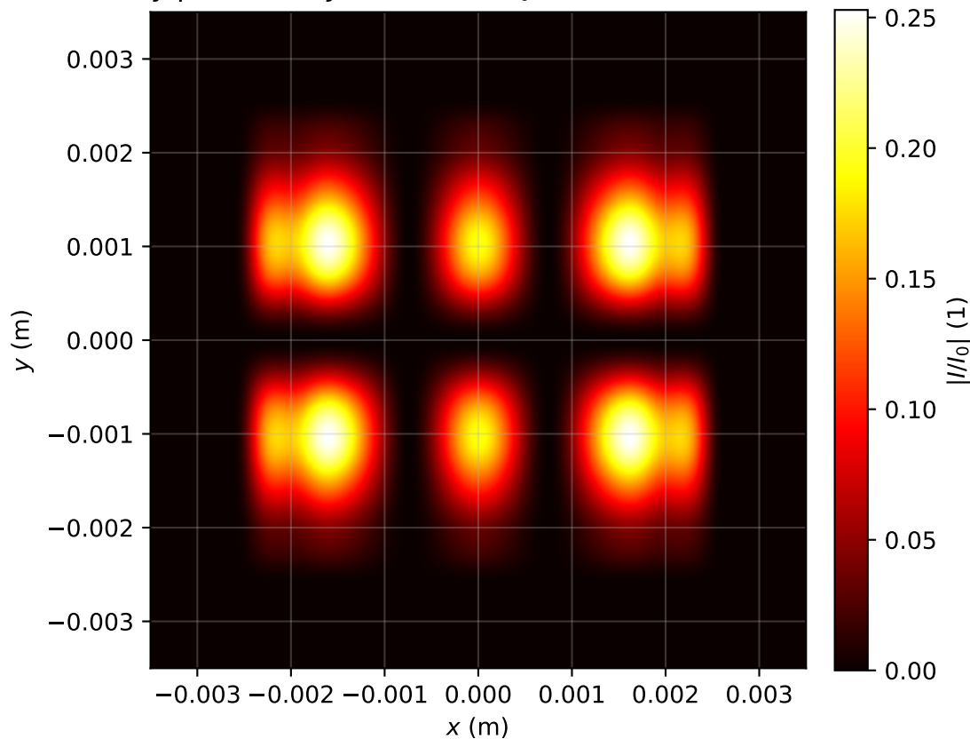
Intensity profile I(x, y, z = 3.662)/I_0 , P_{in}=0.5P_{cr} , artificial time
